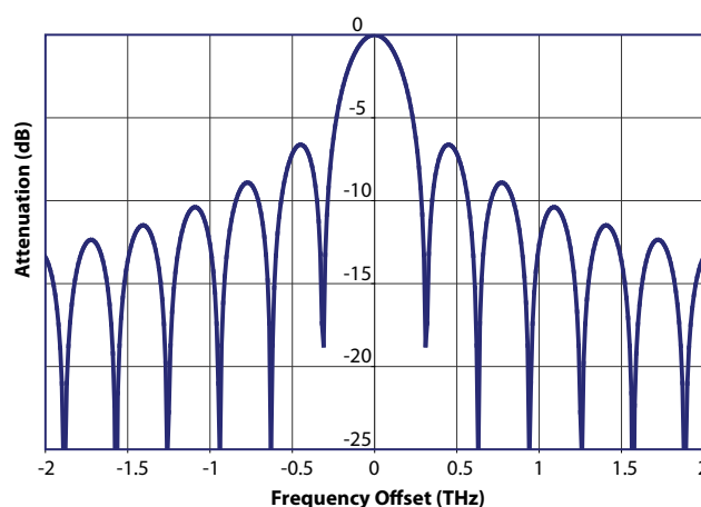
Example filter shapes generated with WaveShaper 1000/4000 programmable optical processor
